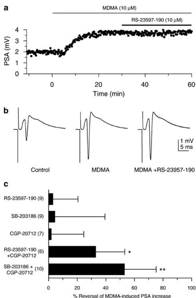
Figure 8 Persistence of ESP_{MDMA} is only partially due to tonic activation of 5-HT_4 and \beta_1 receptors. (a) Time-course plot of a representative experiment in which reversal of N -methyl-3,4-methylenedioxymphetamine (MDMA)-induced PSA increase was attempted by the addition of the 5-HT_4 receptor antagonist, RS-23597-190 ( 10 \mu M ). (b) Data traces from the above experiment. Traces were averaged over the last 20 sweeps recorded in control (left), in MDMA (middle) and in MDMA + RS-23597-190 (right). (c) Bar graph showing the reversal of MDMA-induced population spike amplitude (PSA) increase (mean \pm SD) following 25 to 30-min addition of 5-HT_4 and/or \beta_1 receptor antagonists. In individual experiments, data were normalized so that 0 and 100% reversals correspond to average PSA values obtained during 25–30 min of MDMA application and during the last 5 min before MDMA application, respectively. n values are indicated. * p < 0.05 , ** p < 0.01 (Wilcoxon test).
