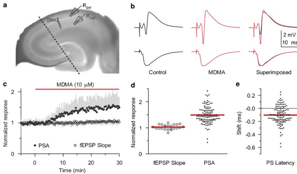
Figure 1 Effects of N -methyl-3,4-methylenedioxamphetamine (MDMA) on population responses. (a) Photomicrograph scheme shows the arrangement of the recording ( R_{\text{rad}} , R_{\text{pyr}} ) and stimulus (S) electrodes in the CA1 region of hippocampal slices. Dotted lines indicate position of a cut made to separate CA1 and CA3 regions. (b) Data traces recorded with electrodes positioned in the stratum pyramidale ( R_{\text{pyr}} , PS (population spikes); above) and in the distal part of stratum radiatum ( R_{\text{rad}} , fEPSP (field excitatory postsynaptic potential); below). Traces were averaged over 20 sweeps recorded immediately before (black lines) and 25–30 min after the beginning of perfusion with 10 \mu\text{M} MDMA (red lines). (c) Summary time–course plot (mean \pm SD; n = 9 from six animals) of MDMA ( 10 \mu\text{M} ) effects on PSA (filled circles) and the fEPSP slope (open circles) recorded as shown above. (d) Scatter plot of effects of MDMA ( 10 \mu\text{M} , 30 min) on PSA and fEPSP slope for all 123 experiments. (e) Scatter plot shows the shift of PSL induced by MDMA ( 10 \mu\text{M} , 30 min) for all experiments.
